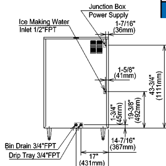
AIR-COOLED UNIT
