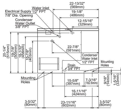
WATER-COOLED UNIT
