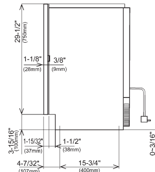
SIDE DIMENSIONS
