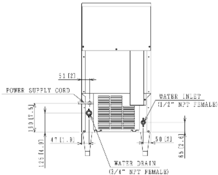
BACK DIMENSIONS
