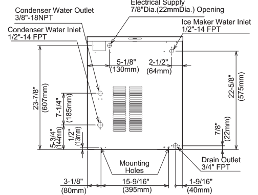
WATER-COOLED UNIT
