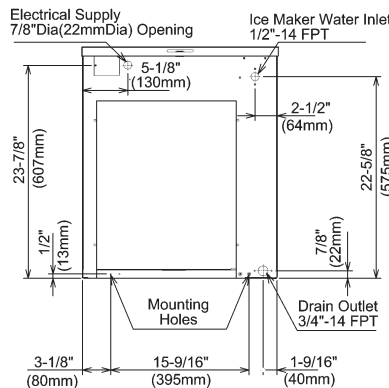
AIR-COOLED UNIT
