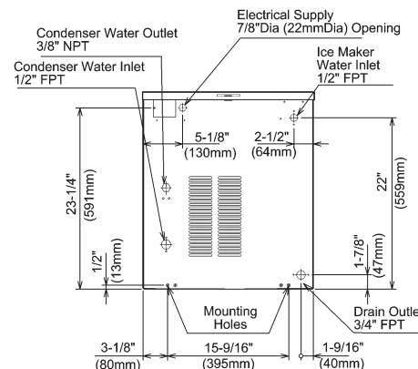
WATER-COOLED UNIT
